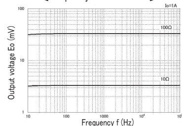
[Frequency characteristics]
