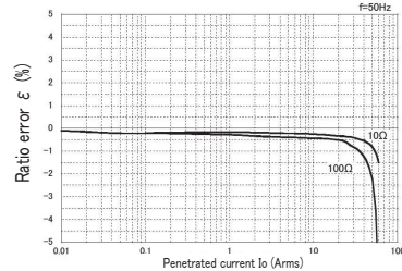
[Ratio error characteristics]
