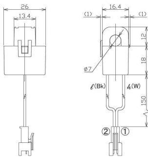
[Outline drawing]
