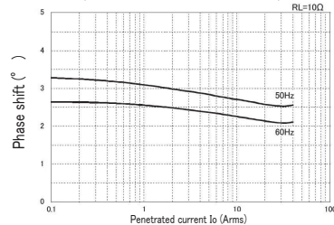
[Phase shift characteristics]
